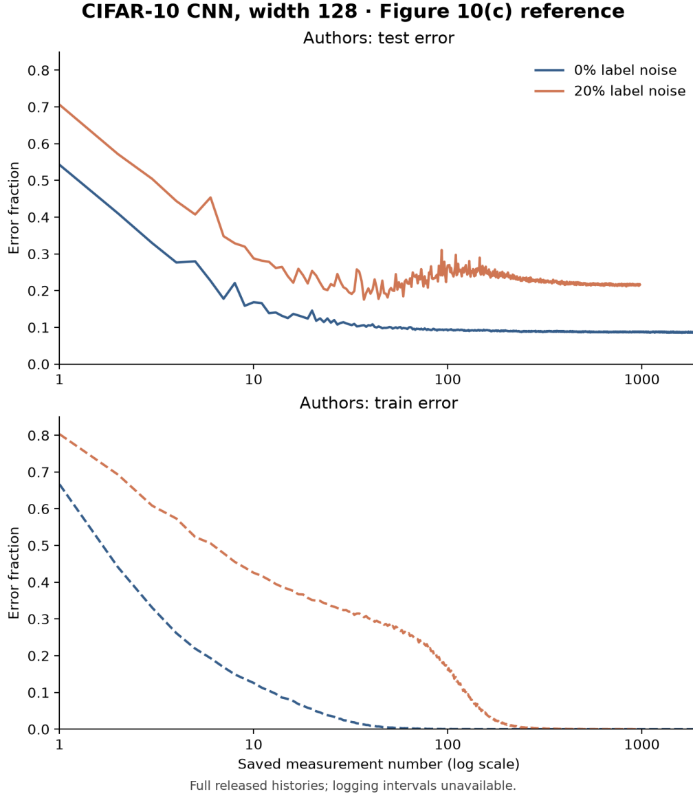
Fig. 19. Authors’ released-data trajectory reconstruction for paper Figure 10(c), showing width-128 clean full-data and 50,000-example 20%-noise sample-grid references on their saved positions rather than model width [1]. Coverage and horizons differ from our reduced runs; see the side-by-side caption and the main-text limitations.
