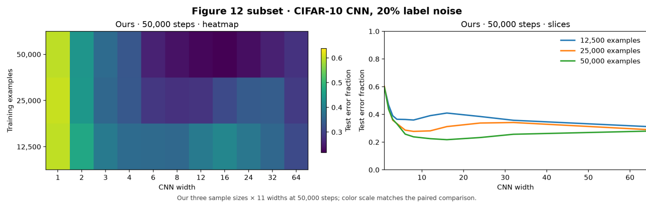
Fig. 11. Our Figure 12 subset: 20%-noise CIFAR-10 CNN sample-size heatmap and slices, using the same color scale as the paired comparison.
