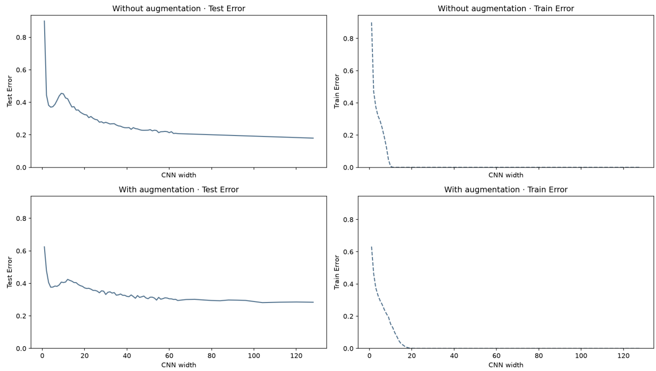
Fig. 15. Authors' released-data reconstruction for paper Figure 5 [1]. Coverage and horizons differ from our reduced runs; see the side-by-side caption and the main-text limitations.
