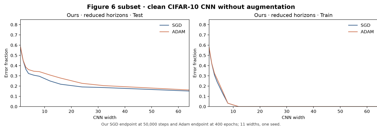
Fig. 6. Our Figure 6 subset: clean, unaugmented CIFAR-10 CNN endpoints for SGD and Adam.
