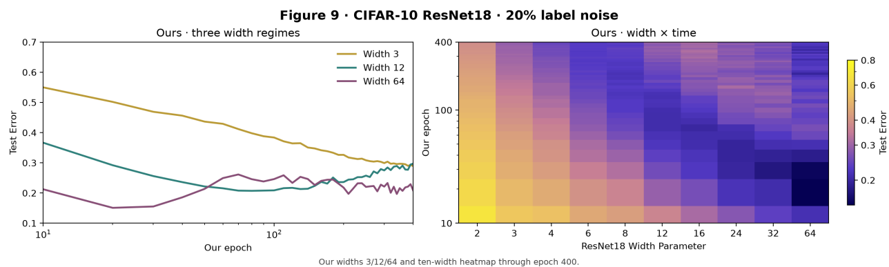
Fig. 8. Our Figure 9 adaptation: 20%-noise CIFAR-10 ResNet18 trajectories and width-by-epoch heatmap.
