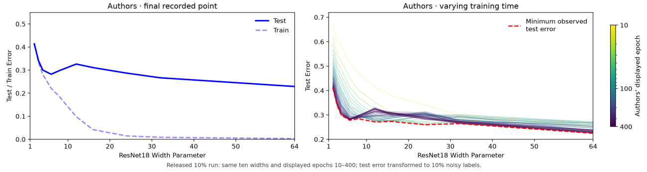
Figure 1 · CIFAR-10 ResNet18 · 10% label noise
