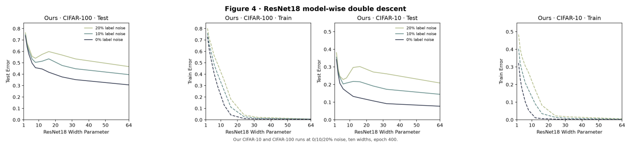
Fig. 4. Our Figure 4 adaptation: CIFAR-10 and CIFAR-100 ResNet18 curves at 0/10/20% noise.
