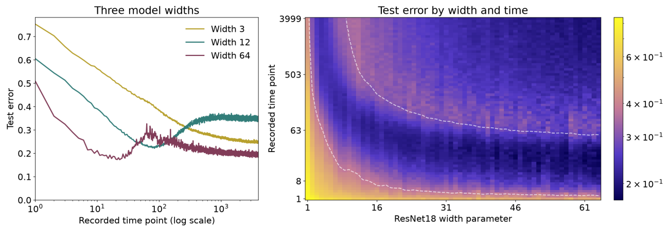
Fig. 18. Authors' released-data reconstruction for paper Figure 9 [1]. Coverage and horizons differ from our reduced runs; see the side-by-side caption and the main-text limitations.
