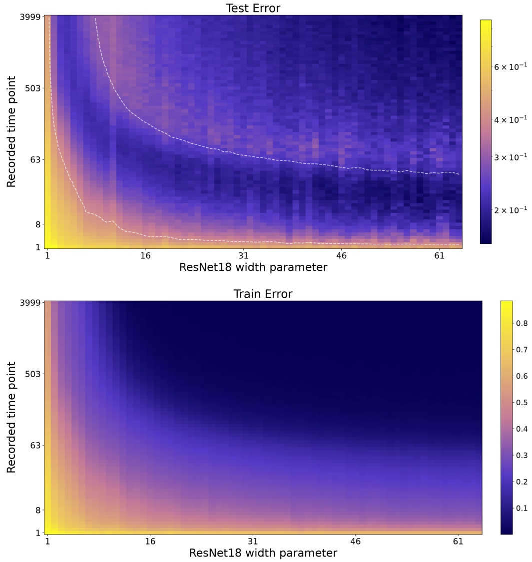
Fig. 13. Authors' released-data reconstruction for paper Figure 2 [1]. Coverage and horizons differ from our reduced runs; see the side-by-side caption and the main-text limitations.
