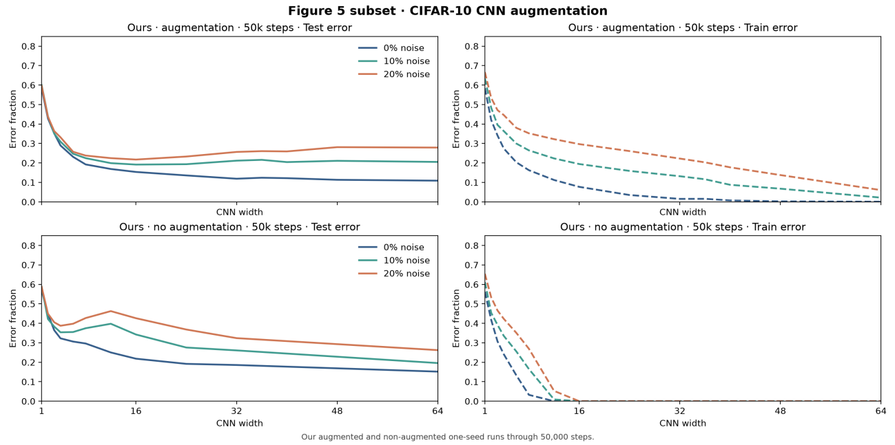
Fig. 5. Our Figure 5 subset: augmented and unaugmented CIFAR-10 CNN curves through 50,000 SGD steps.
