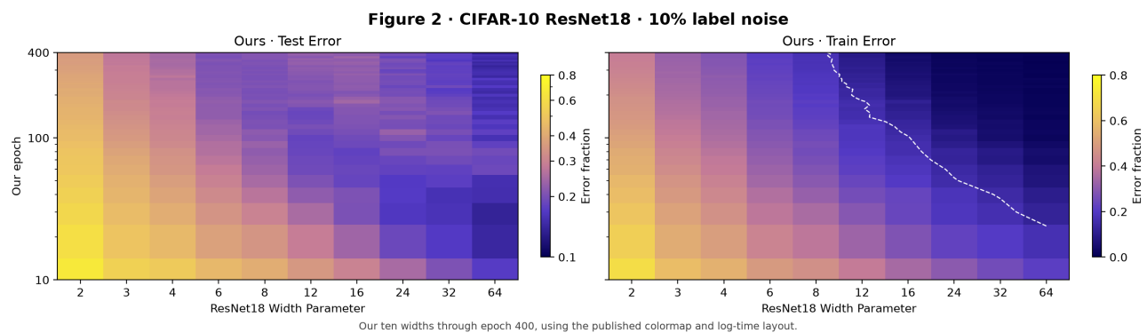
Fig. 3. Our Figure 2 adaptation: 10%-noise CIFAR-10 ResNet18 test and train heatmaps through epoch 400.
