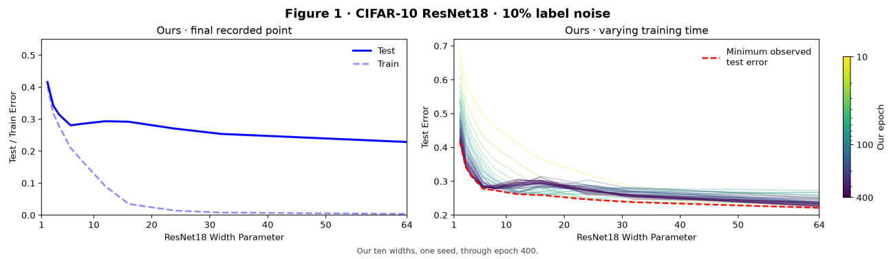
Fig. 2. Our Figure 1 adaptation: 10%-noise CIFAR-10 ResNet18 endpoints and training-time curves through epoch 400.
