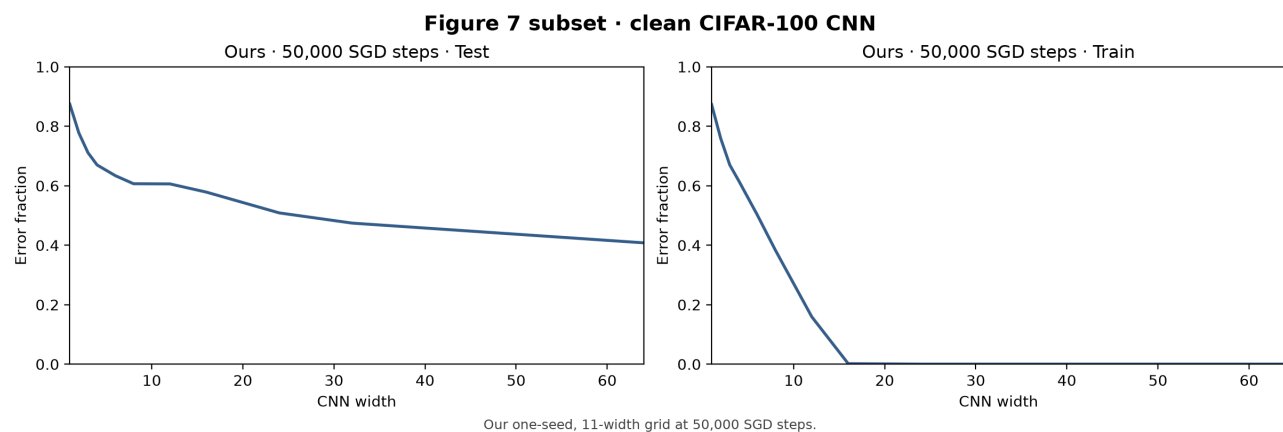
Fig. 7. Our Figure 7 subset: one-seed clean CIFAR-100 CNN endpoints after 50,000 SGD steps.
