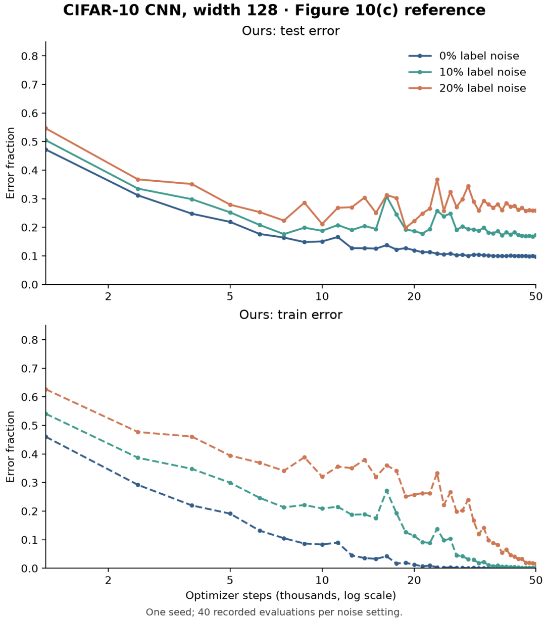
Fig. 9. Our Figure 10(c) subset: width-128 CIFAR-10 CNN test and train histories through 50,000 steps, with all 40 unsmoothed measurements per noise level shown.
