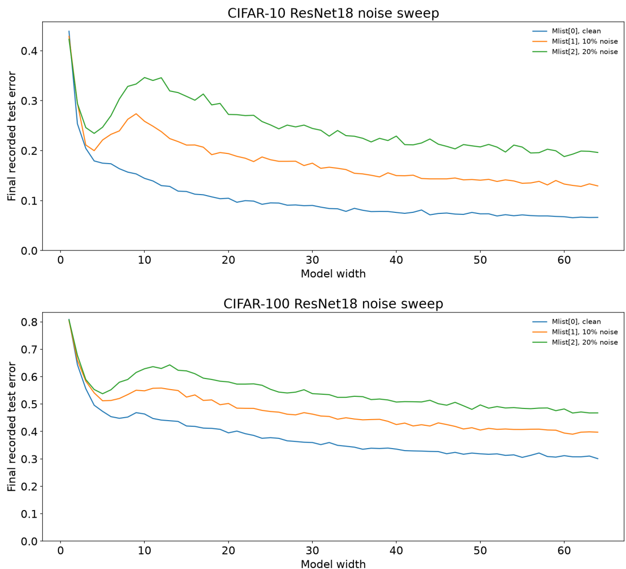
Fig. 14. Authors' released-data reconstruction for paper Figure 4 [1]. Coverage and horizons differ from our reduced runs; see the side-by-side caption and the main-text limitations.
