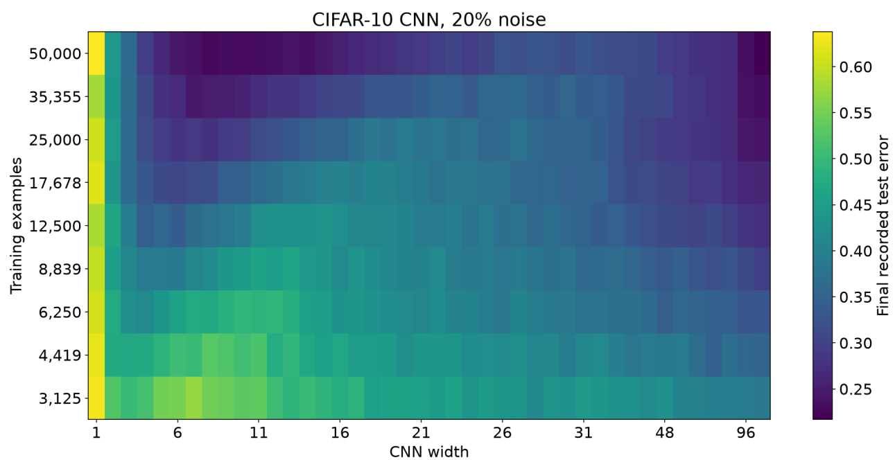
Fig. 21. Authors' released-data reconstruction for paper Figure 12 [1]. Coverage and horizons differ from our reduced runs; see the side-by-side caption and the main-text limitations.
