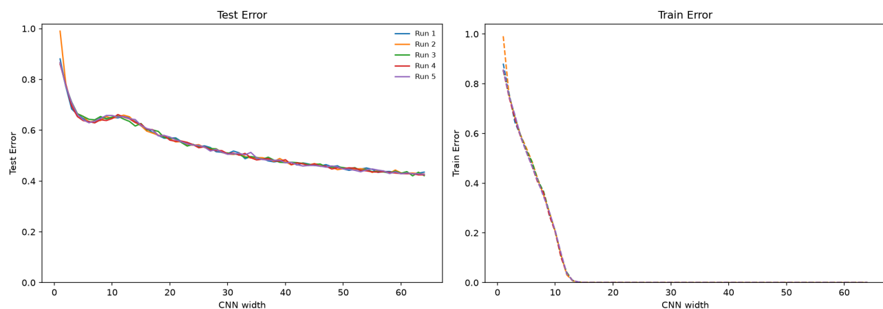
Fig. 17. Authors' released-data reconstruction for paper Figure 7 [1]. Coverage and horizons differ from our reduced runs; see the side-by-side caption and the main-text limitations.
