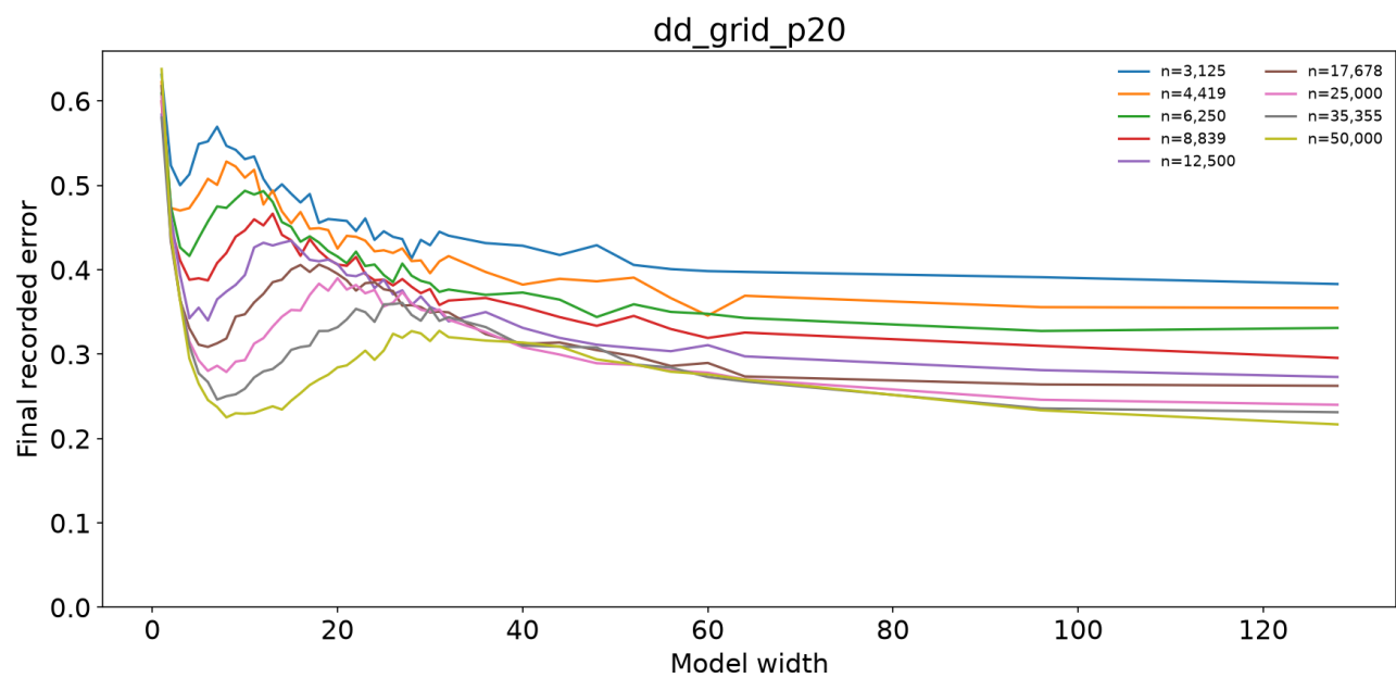
Fig. 20. Authors' released-data reconstruction for paper Figure 11(a) [1]. Coverage and horizons differ from our reduced runs; see the side-by-side caption and the main-text limitations.
