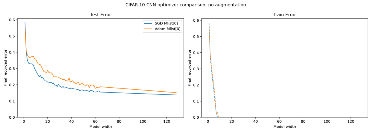
Fig. 16. Authors’ released-data reconstruction for paper Figure 6 [1]. Coverage and horizons differ from our reduced runs; see the side-by-side caption and the main-text limitations.
